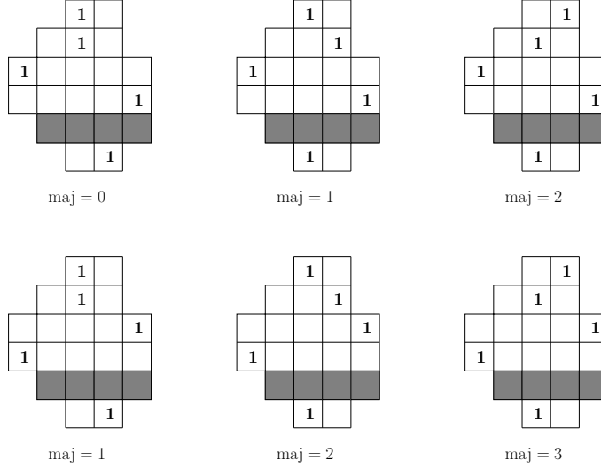
Figure 7: Illustration of Theorem 4.1.
